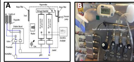
Fig. 2. Nitric Oxide Delivery System for Preclinical Studies. (A) Schematic design of NO chamber. (B) The NO, medical air, N 2 , and CO 2 gas dilution manifold with regulators and digital flowmeters to allow accurate blending and delivery of up to 4 different gases. NO is blended from either a 5000ppm cylinder or AIT NO Generator (NOGen).
