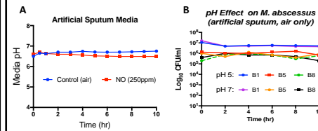
Fig. 6. Effect of culture media pH on M. abscessus viability. (A) Exposure to exogenous NO has been shown to reduce the pH of culture media. Data showing effect of NO exposure on artificial sputum media pH levels in 10hr. (B) Effect of reduced pH on M. abscessus viability was tested. Artificial sputum at pH 5.0 had minimal effect on viability and growth of M. abscessus B1, B5, and B8 clinical strains. This confirms the fact that anti-mycobacterial activity of NO is not caused by minute reductions in pH in artificial sputum media.
