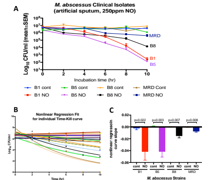
Fig. 7. Antibacterial activity of high-dose NO against multidrug-resistant M. abscessus clinical isolates. (A) Time-kill curves show susceptibility of M. abscessus B1, B5 (smooth), B8 (rough), and MRD (rough) clinical isolates, cultured in artificial sputum, to continuous 250ppm NO treatment. All M. abscessus strains show susceptibility to NO treatment. Controls were exposed to humidified air alone inside the NO chamber. (B) Non-linear regression fit of individual time-kill assays performed on B1, B5, B8, and MRD strains in control (C) and 250ppm NO (NO) is plotted. Mean slope values are plotted in panel C. Unpaired t-test of regression line slopes shows significant difference between control and NO-treated M. abscessus clinical isolates (p values shown in table).
